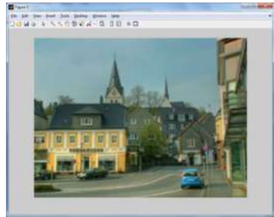
Figure 5: Extracted image
