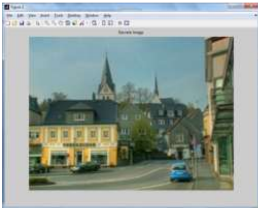
Figure 2: Secret image
