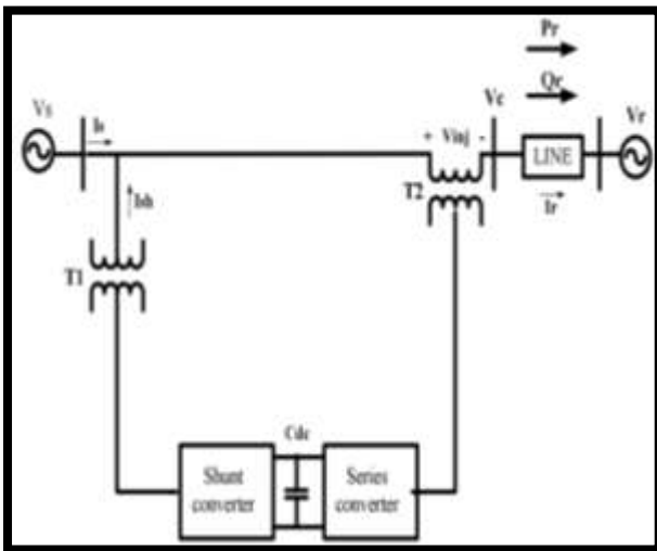
Figure 1. Conventional UPFC consist of shunt and series converters
