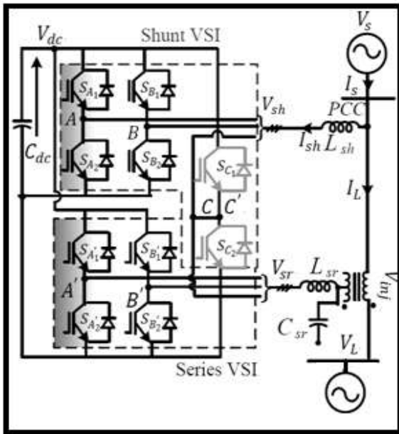
Figure 2: Proposed ten-switch UPFC.
