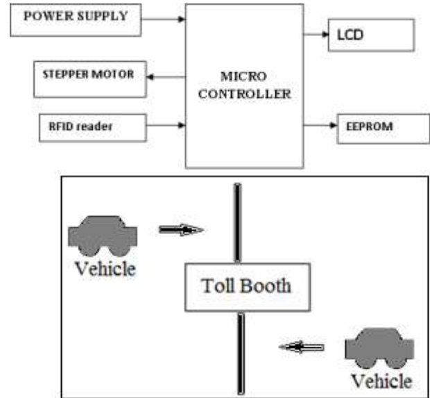
Figure 4: Toll gate management section.
