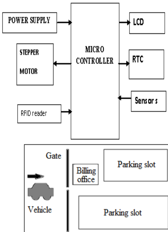
Figure 3: Parking slot management section.
