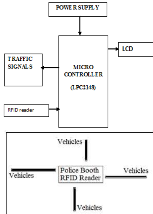
Figure 2: Traffic signal control section.
