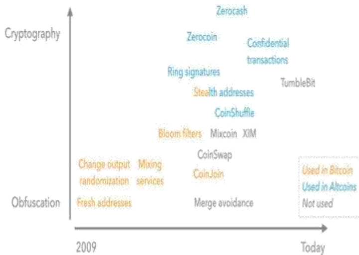
Figure 1: Privacy-Enhancing Technologies for Bitcoin. The X-axis is the date of invention and the Y-axis is an informal measure that combines the sophistication of the technique and the strength of the privacy guarantee. See Appendix 1 for references and dates. 2
