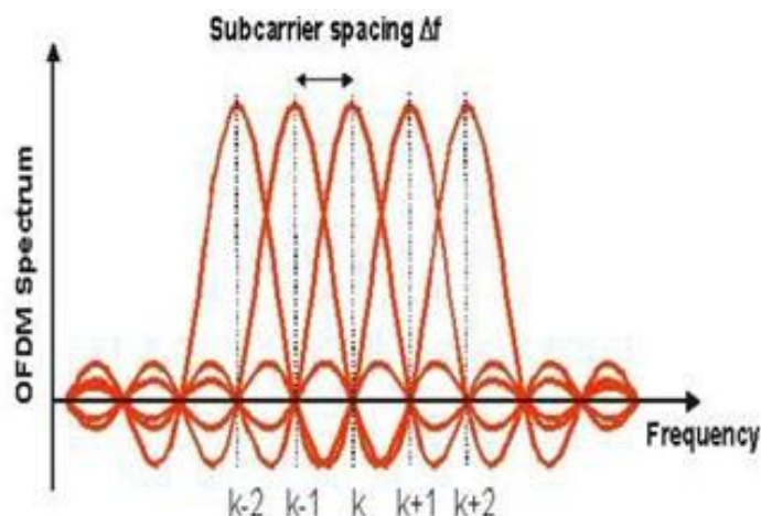
Fig 2: OFDM system using Companding Technique
