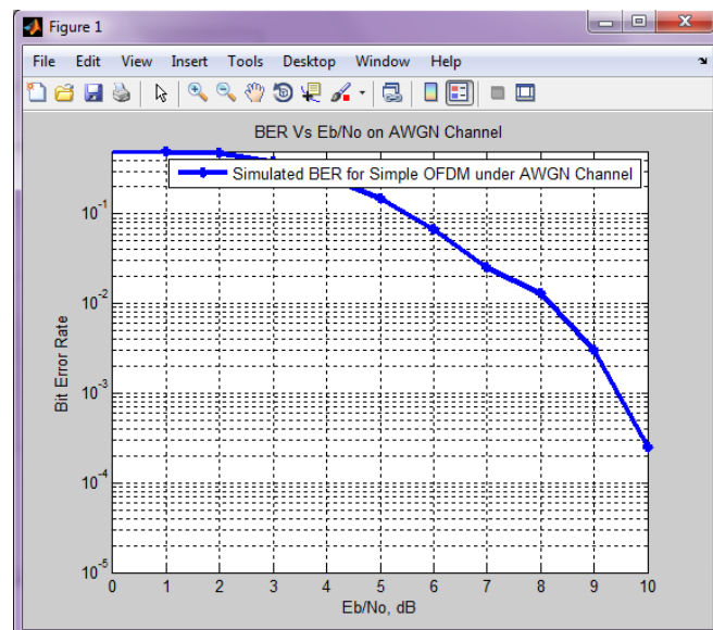
Figure 3 : Simulated BER for Simple OFDM under AWGN Channel.
