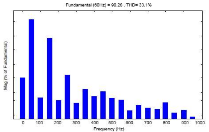
Figure 8: Harmonic Spectrum and THD value of open loop source current under unbalanced condition.
