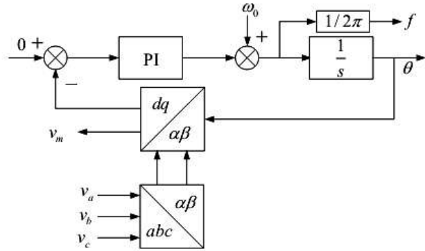
Figure 2: Block diagram of SF-PLL
