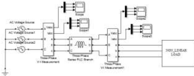
Figure 4: Simulation for open loop system.
