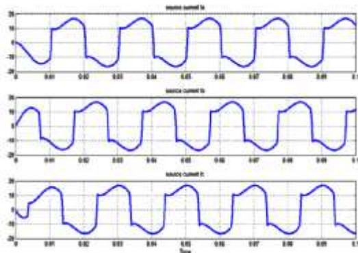
Figure 6: Simulation Waveform for open loop source current.
