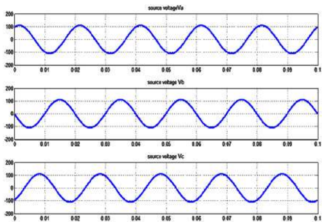
Figure 10: Simulation Waveform for source voltage using PI controller.
