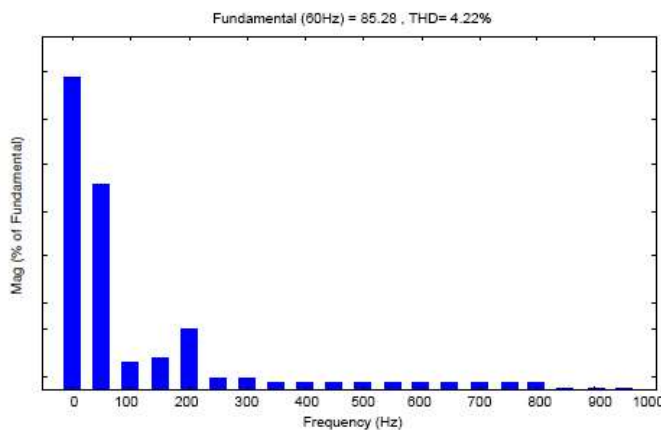
Figure 14: Harmonic spectrum using PI controller with unbalanced condition
