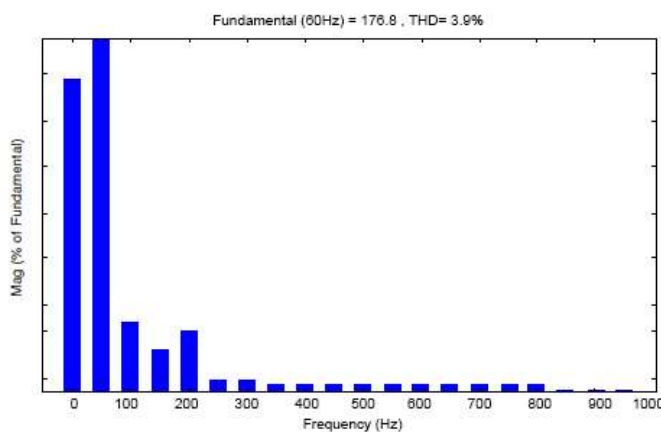
Figure 13: Harmonic Spectrum using PI controller with balanced condition.
