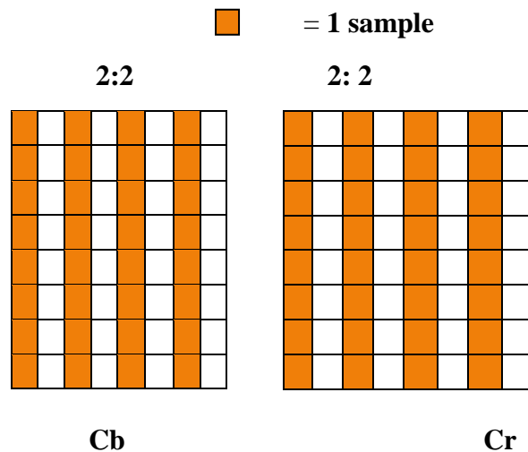
Fig. Block diagram of 2 \times 2 pixel Chroma Subsampling technique.
