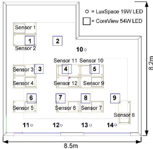
Fig. 1. Layout of two types of LED luminaires in the test bed.
