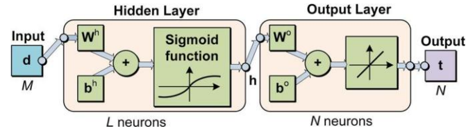
Fig. 8. Two-layer feedforward neural network.
