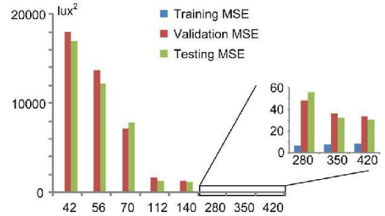
Fig. 12. MSE for different numbers of data sets for training and L = M = 70 .
