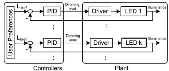
(b) Closed-loop control with multiple SISO approach
