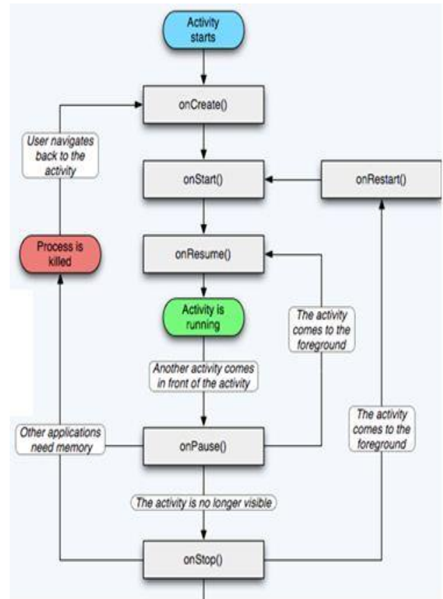
Fig. 1 Activity Life Cycle ( android)
