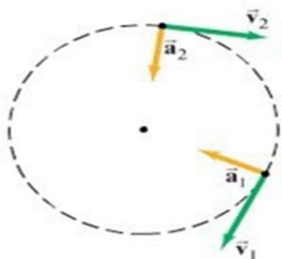
Fig. 2: Centripetal acceleration.
