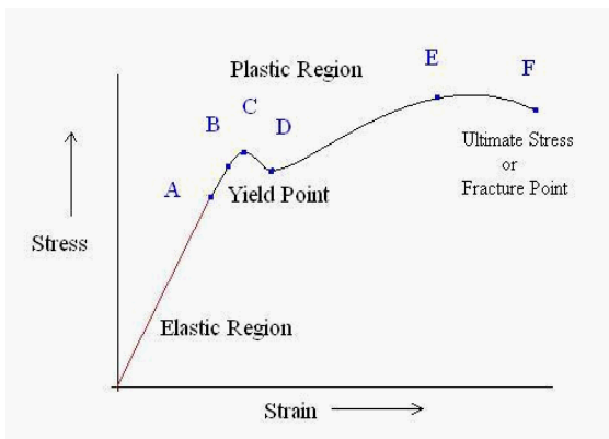
Fig. 4: Stress-strain diagram [6].
