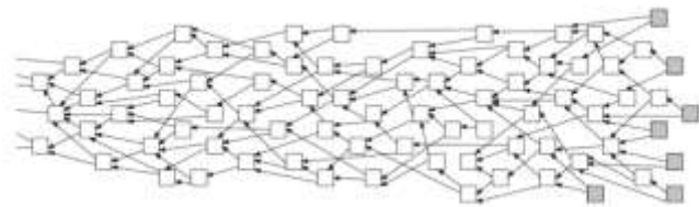
Fig 3.1: Tangle network
