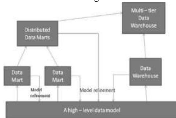
Figure2: Implementation of Data Warehouse in incremental and evolutionary manner.
