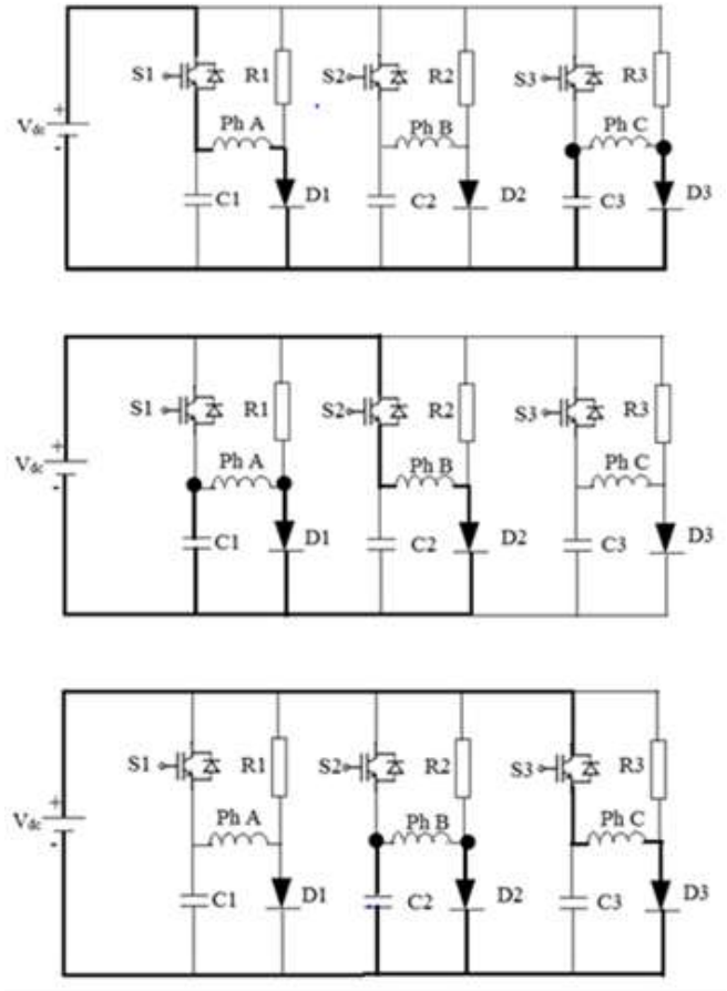
Fig.5. Operating Modes of the Proposed Compact Converter
