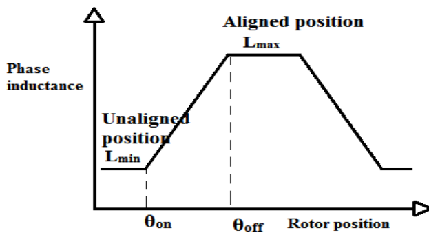
Fig. 2. Inductance profile of SRM
