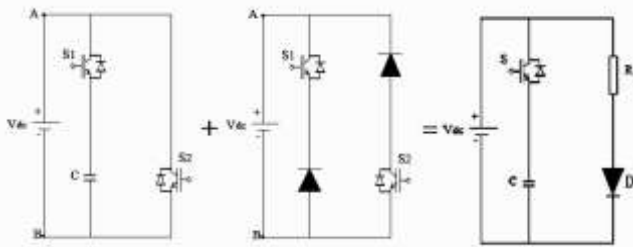
Fig.4. Schematic Diagram of the Proposed Compact Converter
