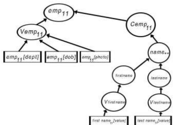
Figure 3: BN to compute similarity of trees in Fig. 1.
