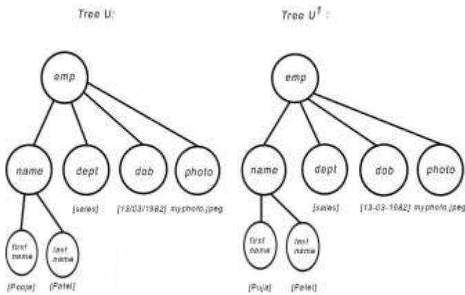
Figure. 1: Two XML elements that represent the same Employee. Nodes are labelled by their XML tag name.
