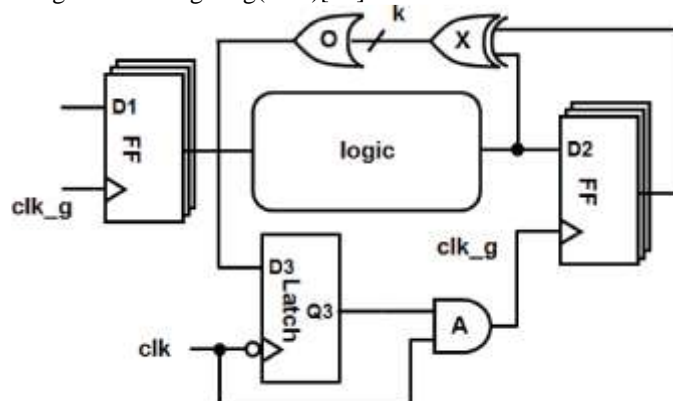
Fig 3 Integrated clock gating applied to group of flipflops
