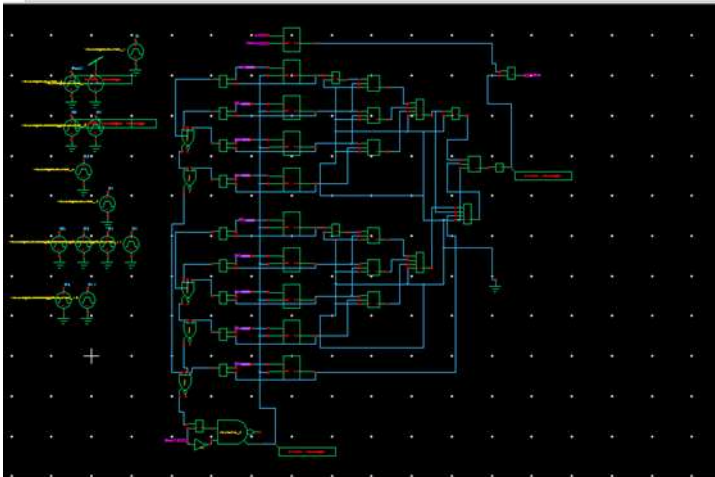
Fig 4. Integrated clockgating for flipflops and their outputs processed in combinational logic in tanner S-edit
