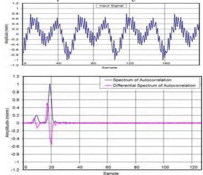
Fig.3 Representation of a speech signal sample and magnitude of the autocorrelation spectrum.
