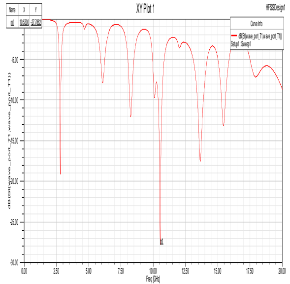
Fig.8 Frequency Vs return loss plot for Circular patch antenna
