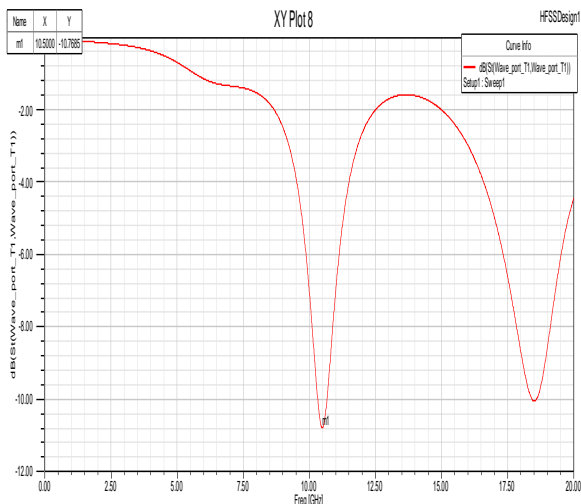
Fig 2. Frequency Vs return loss plot for rectangular patch antenna
