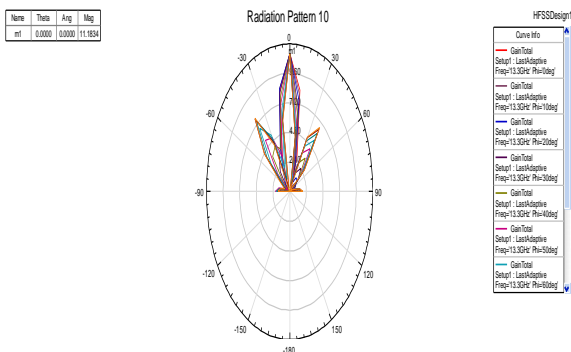
Fig.12 Radiation Pattern for C slot Circular patch antenna
