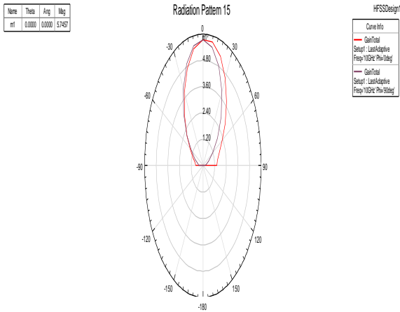
Fig 6. Radiation Pattern for C slot rectangular patch antenna
