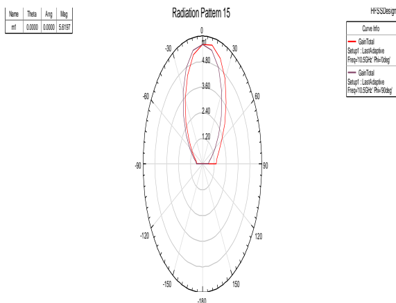
Fig 3. Radiation Pattern for rectangular patch antenna
