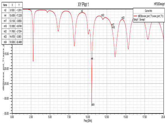
Fig 11. Frequency Vs return loss plot for C slot Circular patch antenna
