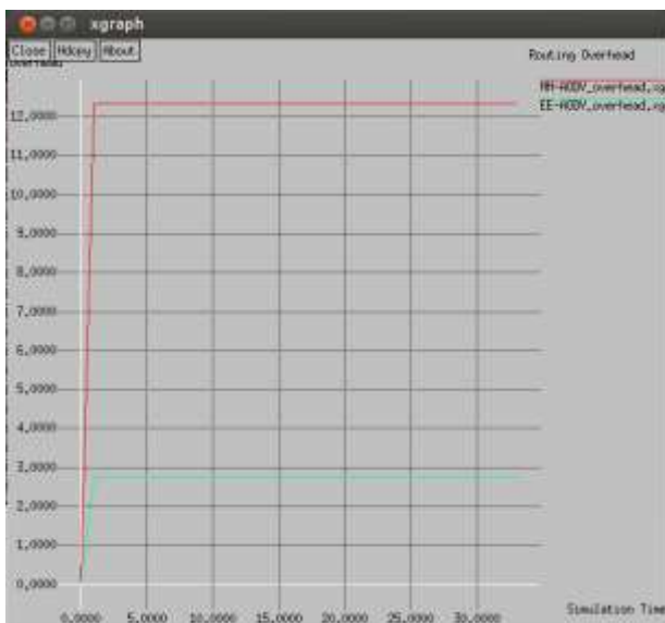
Fig 3: Routing overhead vs Simulation time
