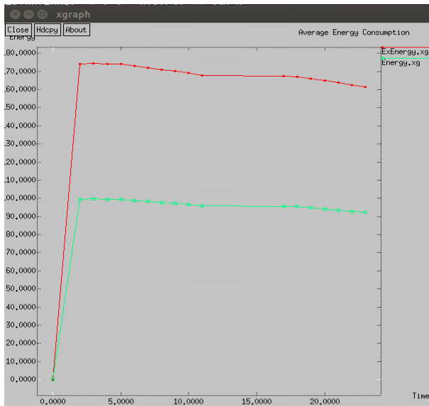
Figure 4 Energy Consumption
