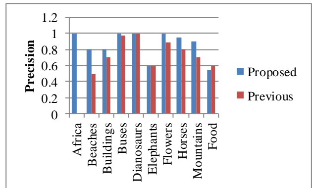
Figure 6: Precision Comparison
