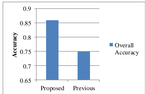
Figure 7: Accuracy Comparison
