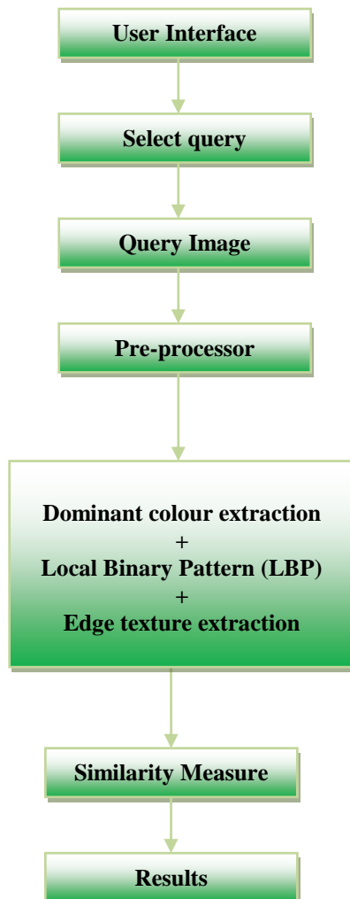
Figure 1: Architecture
