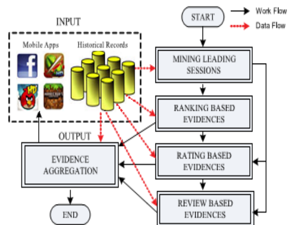
Fig. 1 The framework of our ranking fraud detection system for mobile Apps.
