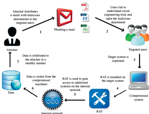
Fig. 1: Phishing Attack
