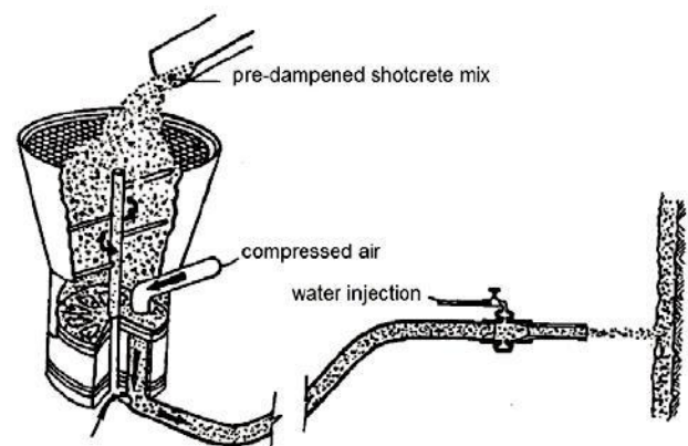
Figure 1. Simplified sketch of a typical dry mix
