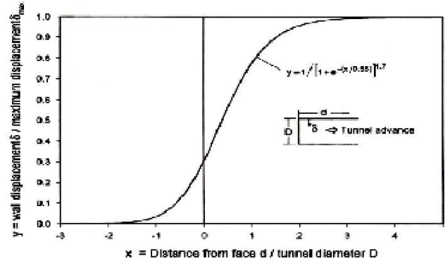
Figure 6. Tunnel displacement or stress discharged before installing the support.
