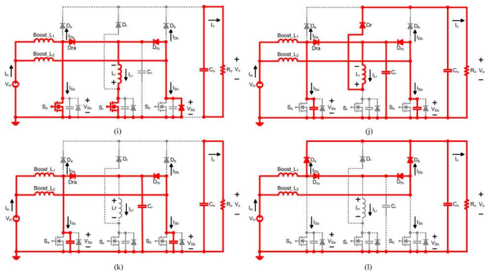
Fig. 4 Equivalent circuits of different modes ( D < 50\% ). (a) Mode 1 [ t_0-t_1 ]. (b) Mode 2 [ t_1-t_2 ]. (c) Mode 3 [ t_2-t_3 ]. (d) Mode 4 [ t_3-t_4 ]. (e) Mode 5 [ t_4-t_5 ]. (f) Mode 6 [ t_5-t_6 ] (g) Mode 7 [ t_6-t_7 ]. (h-a) Mode 8 [ t_7-t_a ]. (h-b) Mode 8 [ t_a-t_8 ]. (h-c) Detailed waveform of the Mode 8. Equivalent circuits of different modes ( D < 50\% ). (i) Mode 9 [ t_8-t_9 ]. (j) Mode 10 [ t_9-t_{10} ]. (k) Mode 11 [ t_{10}-t_{11} ]. (l) Mode 12 [ t_{11}-t_{12} ].
