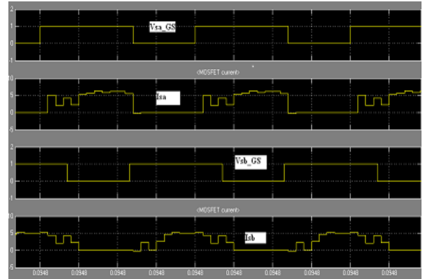
Fig. 12 Simulation waveforms of the main switches S_a and S_b ( D > 50\% and load current 1.5A). (a) ZVS. (b) ZCS
