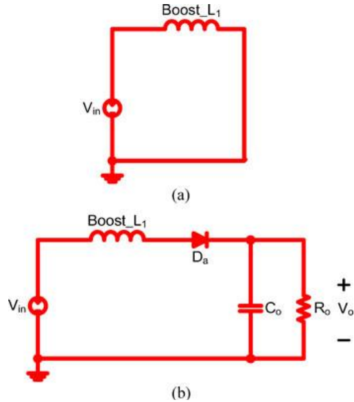
Fig. 6 Equivalent circuits for the boost inductor ( D < 50\% ). (a) Boost_L1 in the stage [t_b-t_c] , stage [t_d-t_e] , stage [t_e-t_f] , stage [t_f-t_g] and stage [t_h-t_i] . (b) Boost_L1 in the stage [t_a-t_b] , stage [t_c-t_d] and stage [t_g-t_h] .
