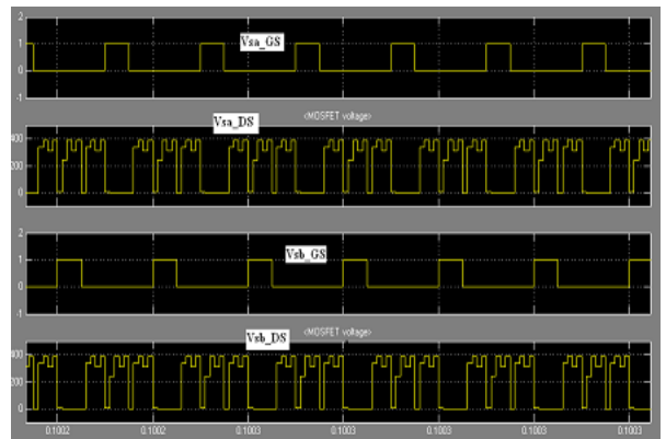
Fig. 13 Simulation waveforms of the main switches S_a and S_b ( D < 50\% ). (a) ZVS. (b) ZCS
