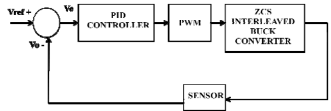
Fig:15 Functional Block diagram of closed loop control of interleaved buck converter
