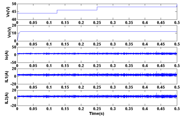
Fig. 16. Simulation results for ZCS Interleaved Buck Converter (V s -Input Voltage, V o -Output Voltage, I o -Load Current, I L1 and I L2 -Inductor Currents)
