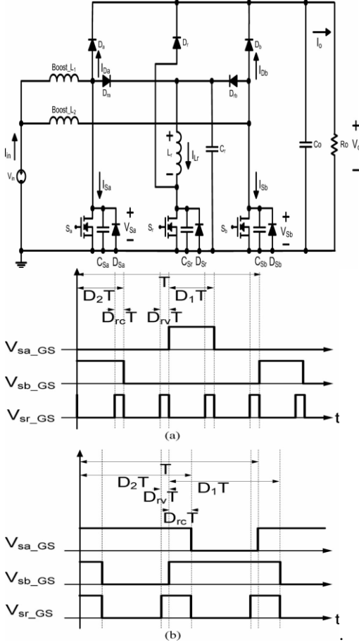
Fig. 2 Switching waveforms of the main switches S_a and S_b and auxiliary switch S_r . (a) D < 50\% mode. (b) D > 50\% mode.
