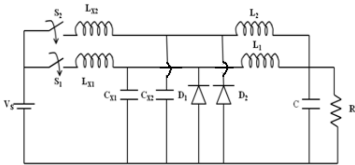
Fig:14-schematic diagram of ZCS interleaved buck converter
