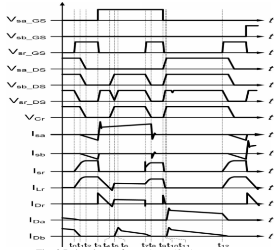
Fig. 3 Related waveforms ( D < 50\% ).
