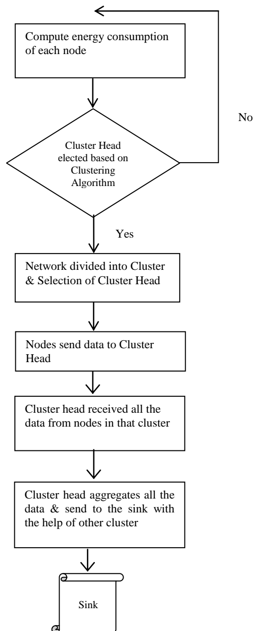
Figure 5. Cluster Formation & data transfer
