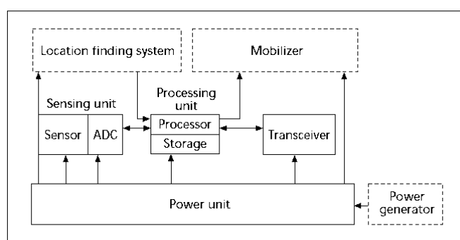
Figure 2. Sensor node components
