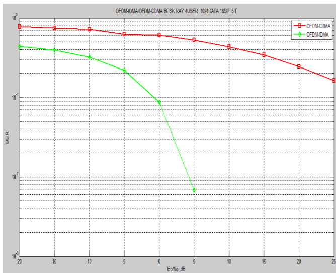
Figure 6: Performance analysis of User 1
