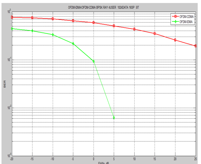
Figure 1: Performance analysis of User 3
