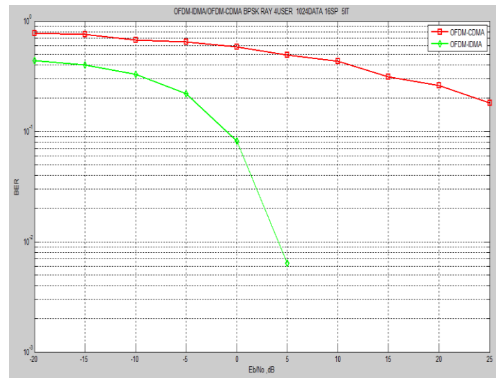
Figure 1: Performance analysis of User 4
