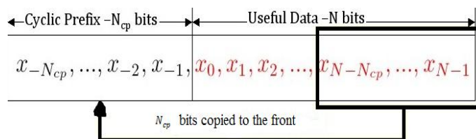
Figure 4: Cyclic-prefix
