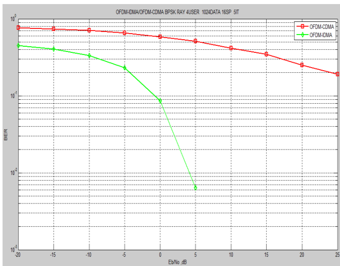
Figure 7: Performance analysis of User 2
