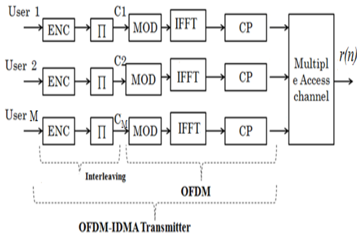
Figure 1:OFDM –IDMA Transmitter
