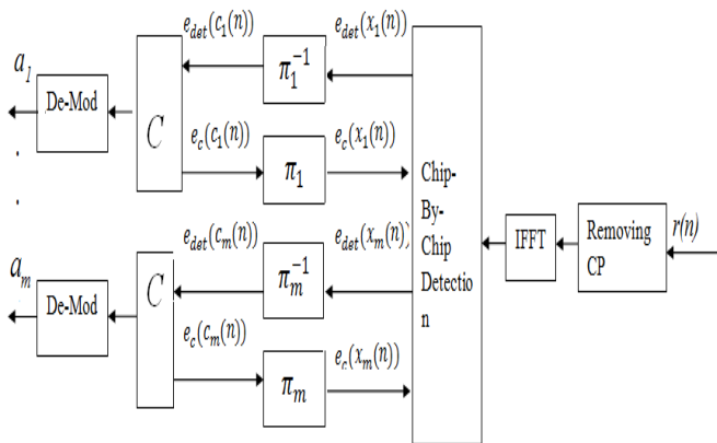
Figure 1: OFDM-IDMA Iterative Receiver
