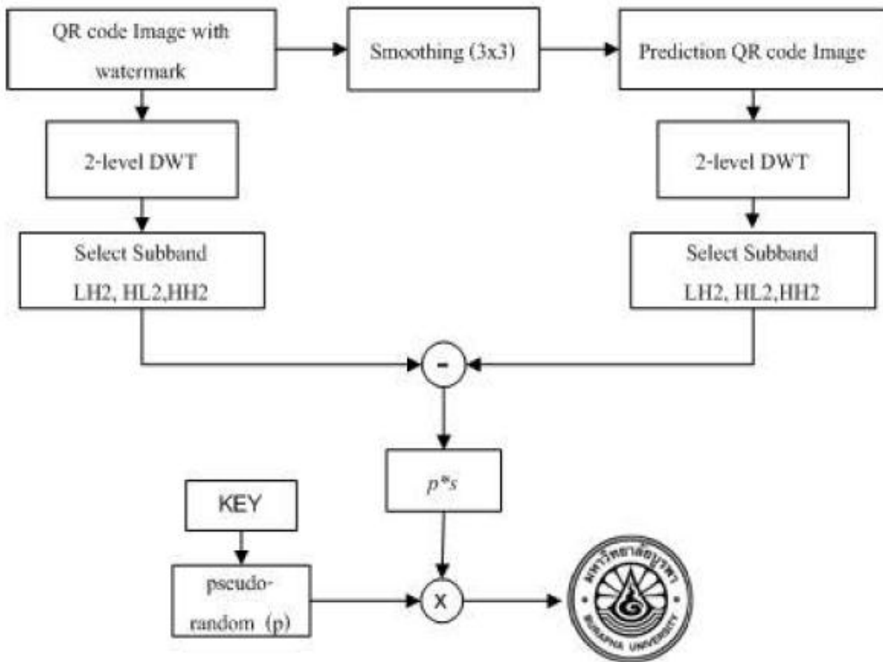
Fig. 4. Watermark Extracting Process
