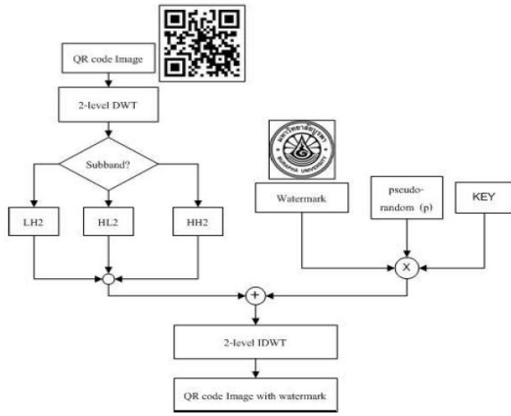
Fig. 3. Watermark Embedding Process
