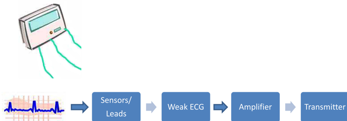
Fig. 4 Sender (ECG monitor) Architecture
